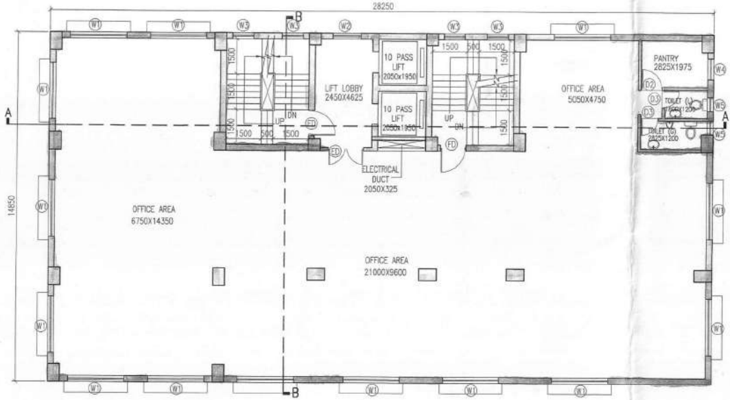
SEVENTH FLOOR PLAN SCALE - 1 : 100
