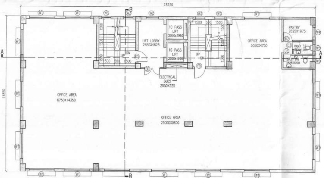
FIFTH & SIXTH FLOOR PLAN SCALE - 1 : 100
