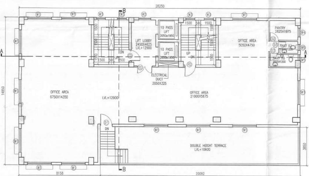
FOURTH FLOOR PLAN SCALE - 1 : 100
